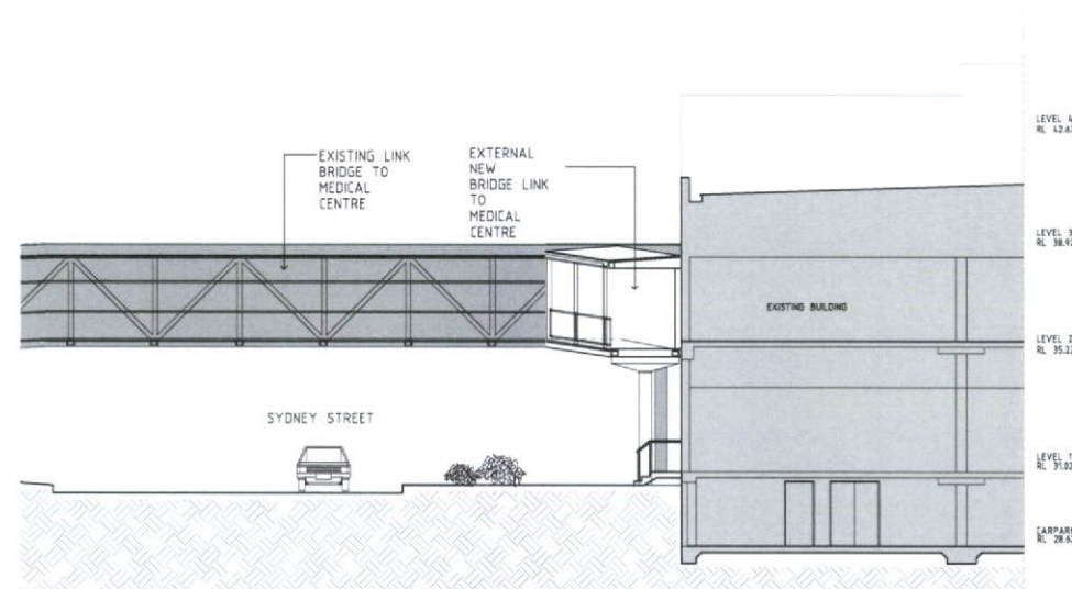
01 - SECTION OF NEW LINK BRIDGE
