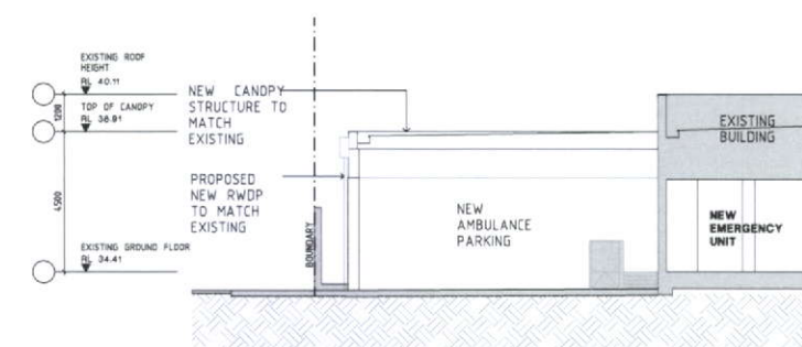
02 - SECTION/NEW CANOPY
