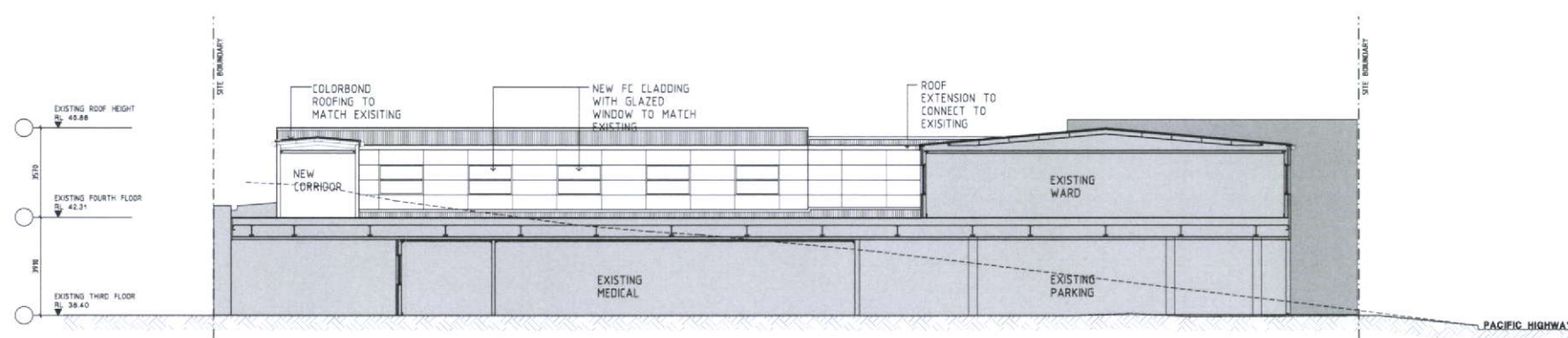
05 - WARD EXTENSION NORTH ELEVATION
