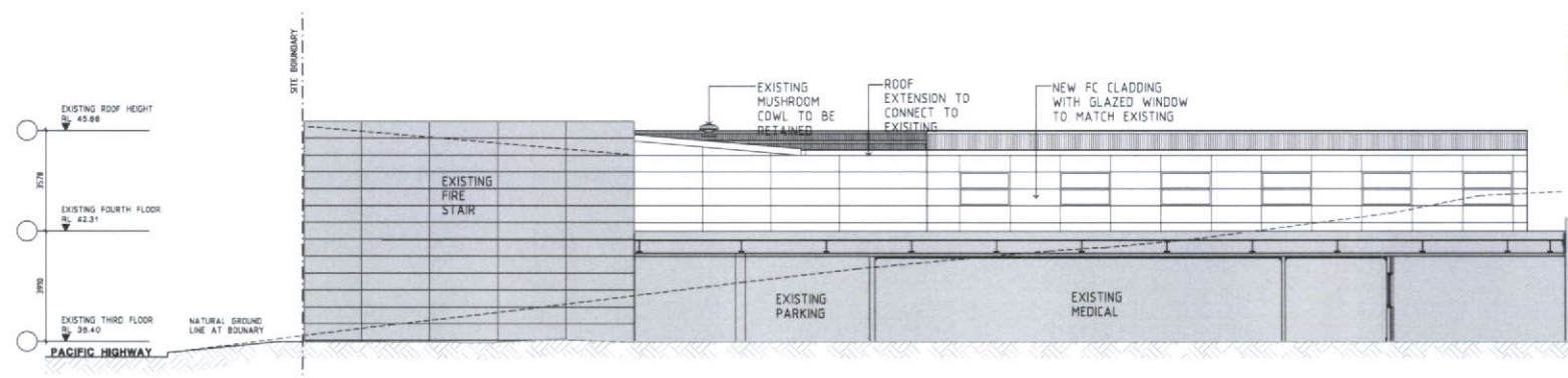
04 - WARD EXTENSION SOUTH ELEVATION
