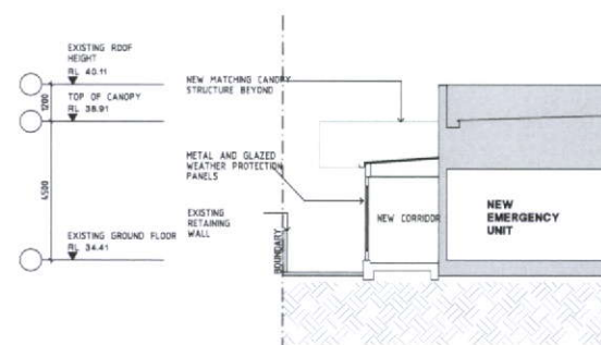
03 - SECTION/ NEW EMERGENCY ACCESS CORRIDOR
