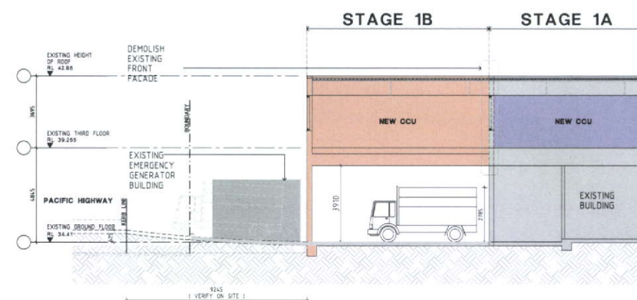
04 - SECTION/ LOADING DOCK
